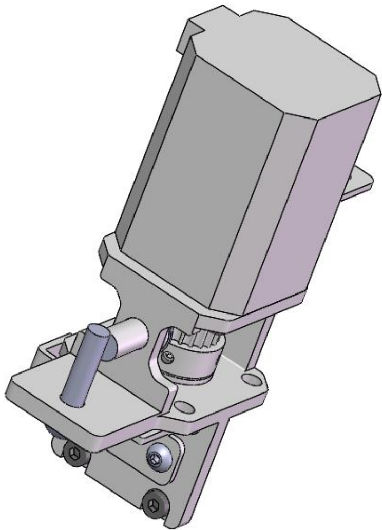
20.205.0104 X电机组件 X-Axis Motor Assembly
