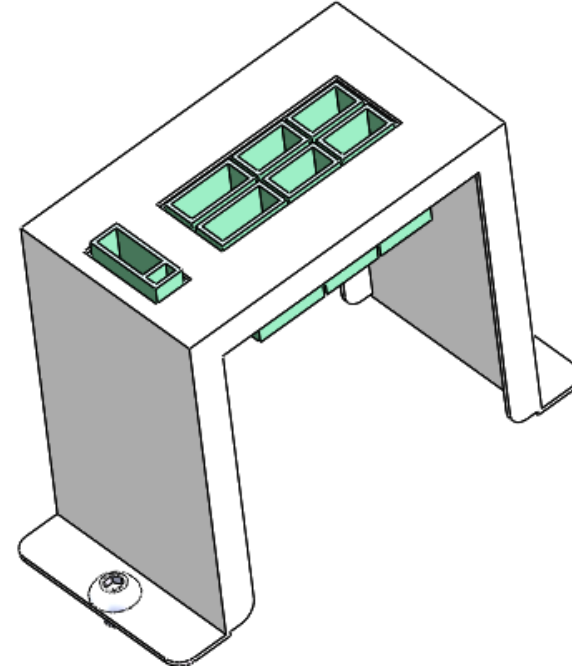
20.205.0098 机箱转接板组件 Chamber Adapter Assembly
