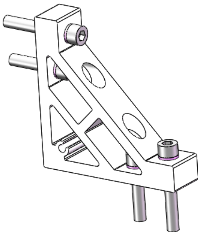
20.204.0176 型材角码组件 (先装) Profile Corner Connector Assembly (Pre- Assembly)
