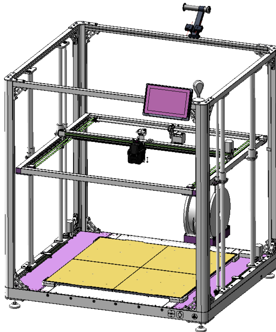
20.202.0038 裸机 Bare Machine
