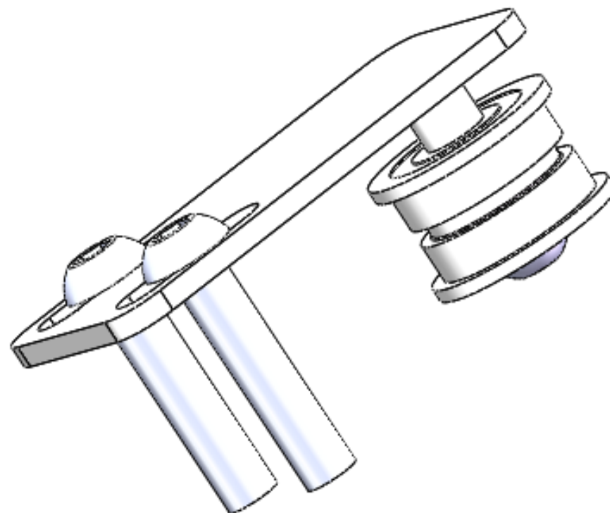
20.204.0173 Z轴张紧组件 Z-Axis Belt Tensioner Assembly
