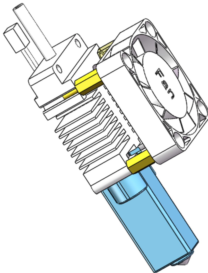
20.206.0034 Nozzle Heatsink Assembly Cat # 001476
