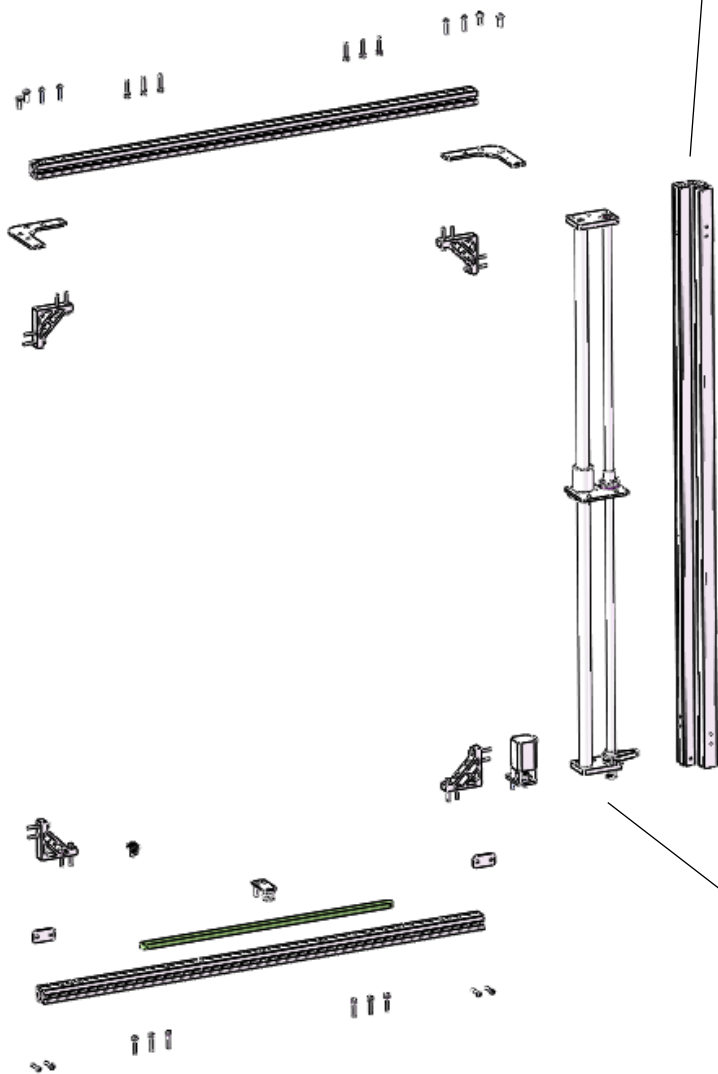
02.203.0088 Z轴左后型材 Z-Axis Left Rear Profile
