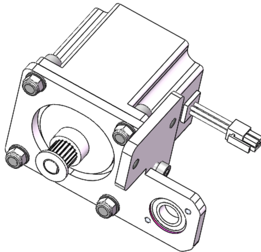
20.204.0178 Y轴电机组件 Y-Axis Motor Assembly
