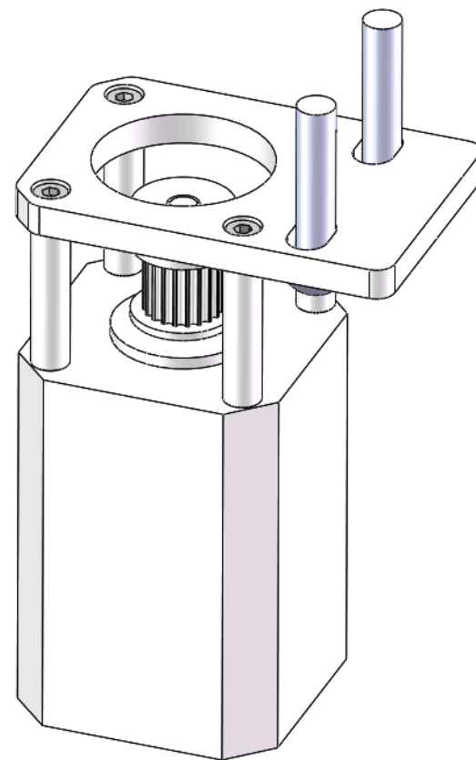
20.204.0174 Z轴电机左组件 Left Assembly of the Z-Axis Motor
